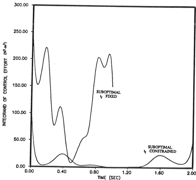
Figure 5: Integrand of Control Effort (Sum of Joint Torques Squared) for Example 1 (Fixed and Constrained Final Time).
