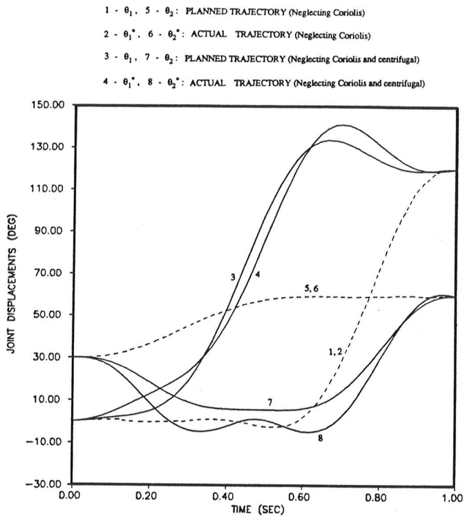
Figure 9: Suboptimal Planned and Actual Displacement Histories for Example 2 (from Figure 8)
