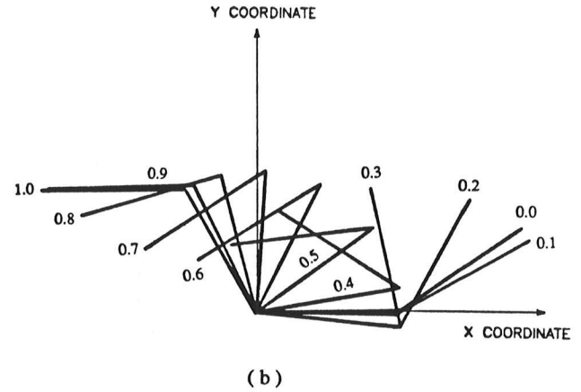
Figure 4: Multiple Exposure Schematic Drawings of Robot Executing (a) Cubic Polynomial Trajectory, and (b) State Unconstrained Suboptimal Trajectory (at 0.1 sec intervals).
