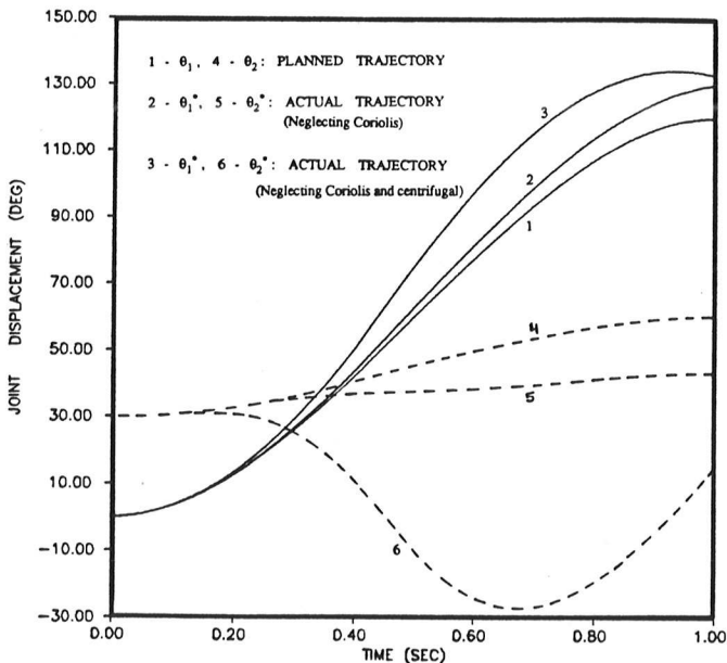
Figure 7: Cubic Polynomial Planned and Actual Displacement Histories for Example 2 (from Figure 6.)
