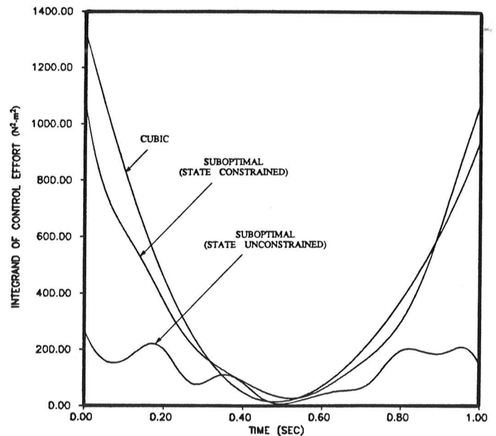
Figure 3: Integrand of Control Effort (Sum of Joint Torques Squared) for Example 1 (Fixed Final Time).
