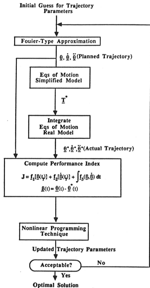
Figure 8: Flowchart of Closed-Loop Algorithm for Generating Suboptimal Planned and Actual Trajectories.
