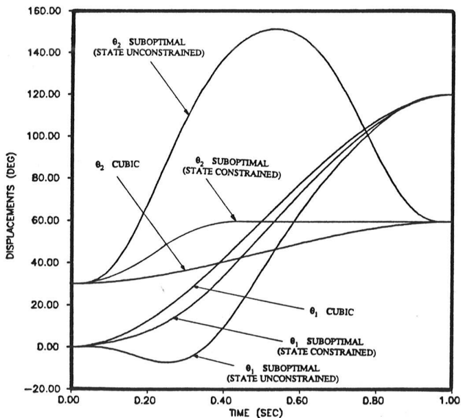
Figure 2: Joint Displacement Histories for Example 1 (Fixed Final Time).
