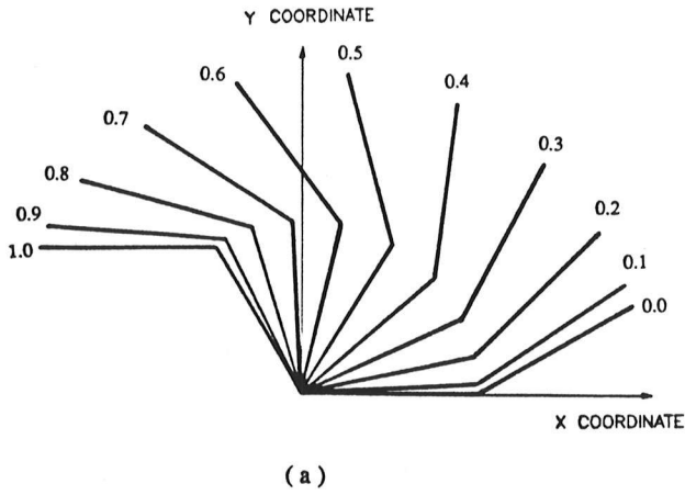
Figure 4: Multiple Exposure Schematic Drawings of Robot Executing (a) Cubic Polynomial Trajectory, and (b) State Unconstrained Suboptimal Trajectory (at 0.1 sec intervals).
