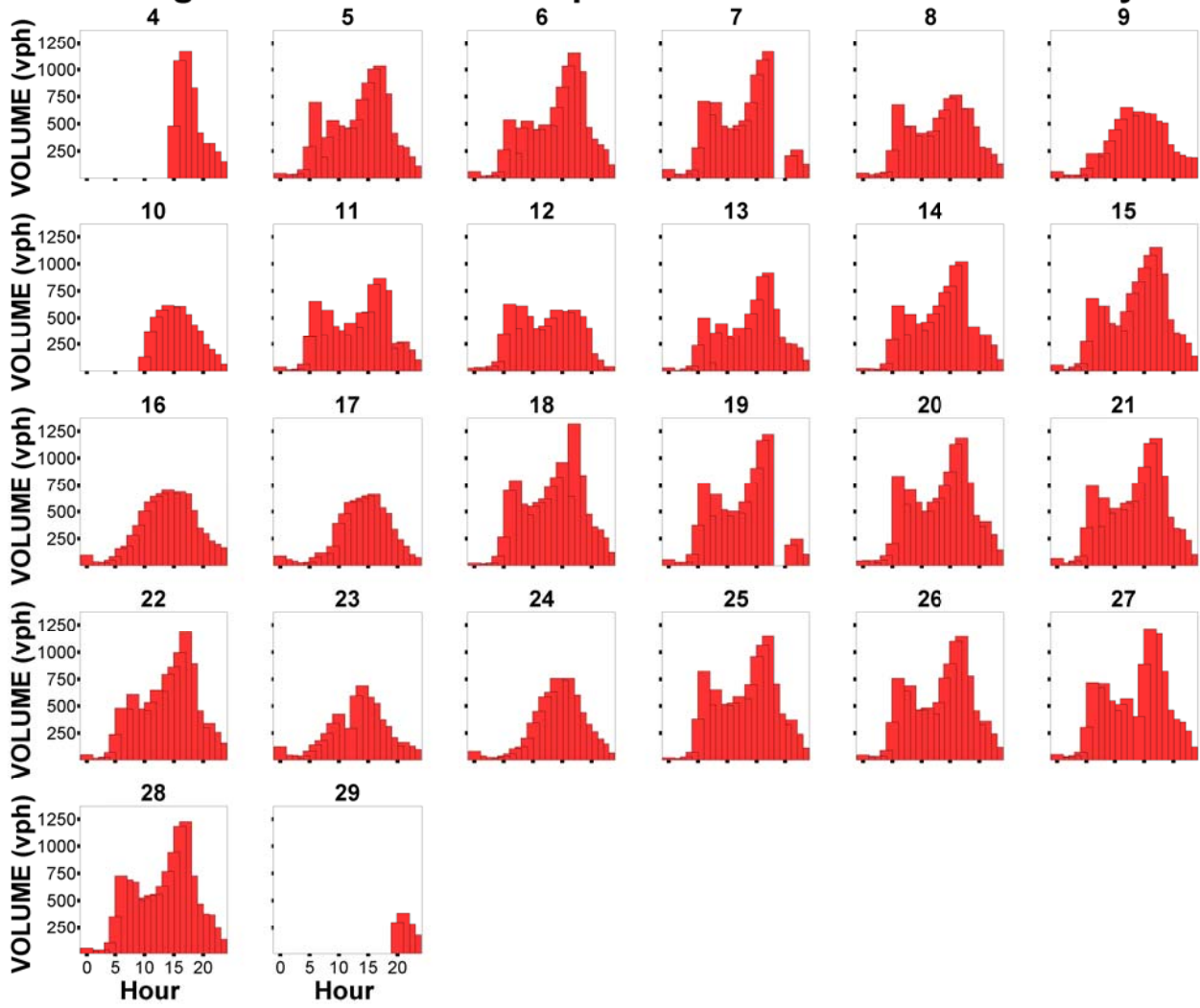
A6 Figure 10. Control Ramp: Detector C Volumes January 1999.
